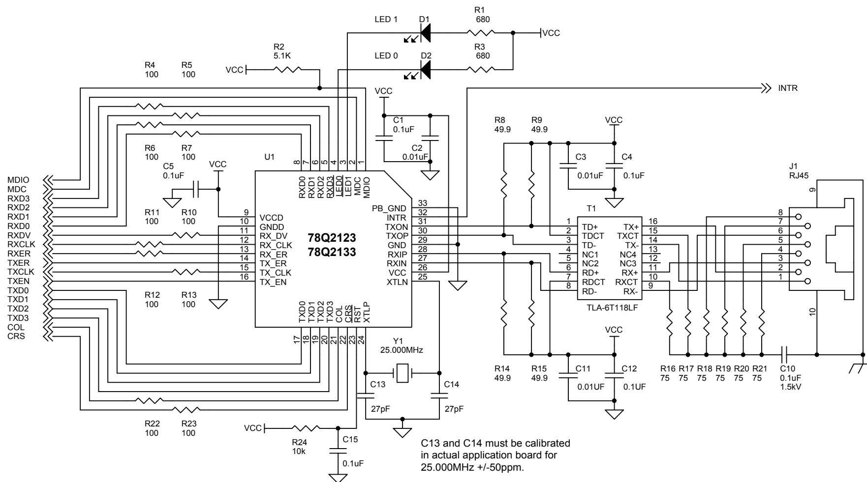
Application Diagram for 78Q2123/78Q2133
