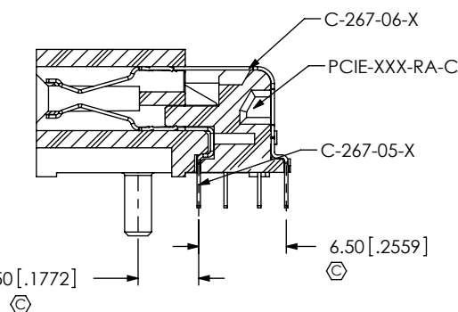
SECTION "B"-"B" (SAME AS SECTION "A"-"A", EXCEPT AS SHOWN)
