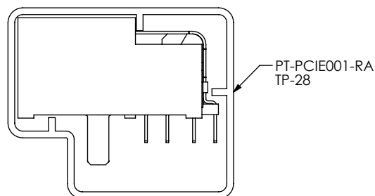
PACKAGING VIEW
