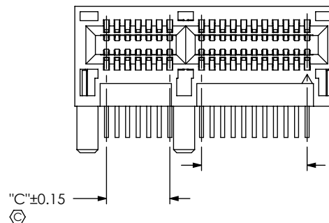
IN-PROCESS 8 (CUT OFF TOP CONTACT CARRIER)
