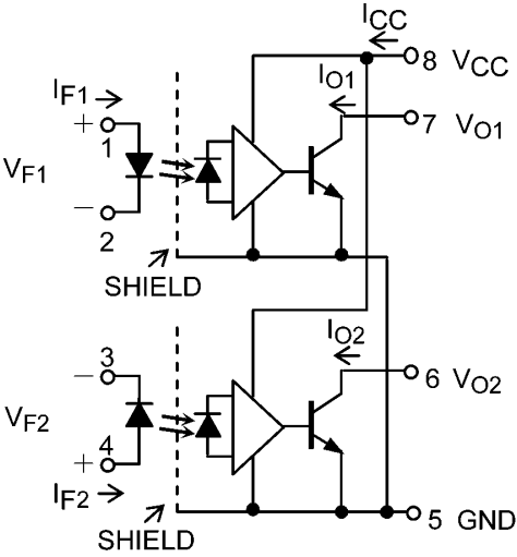
Fig. 5.1 Internal Circuit
