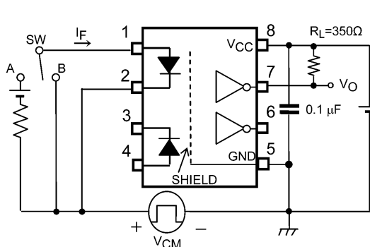
Fig. 12.1.6 Common-Mode Transient Immunity and Waveform
