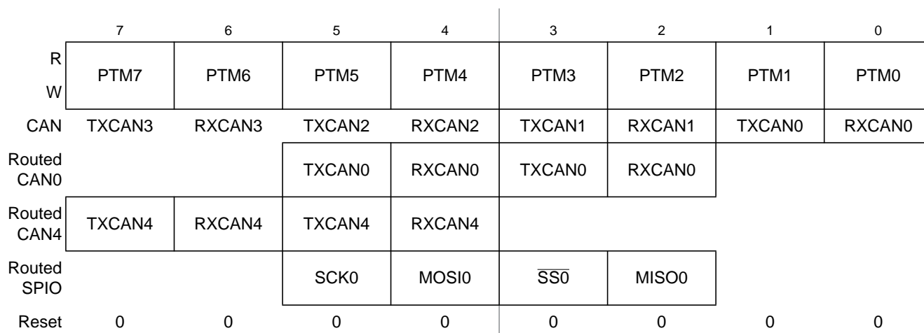
Figure 22-32. Port M Data Register (PTM)
