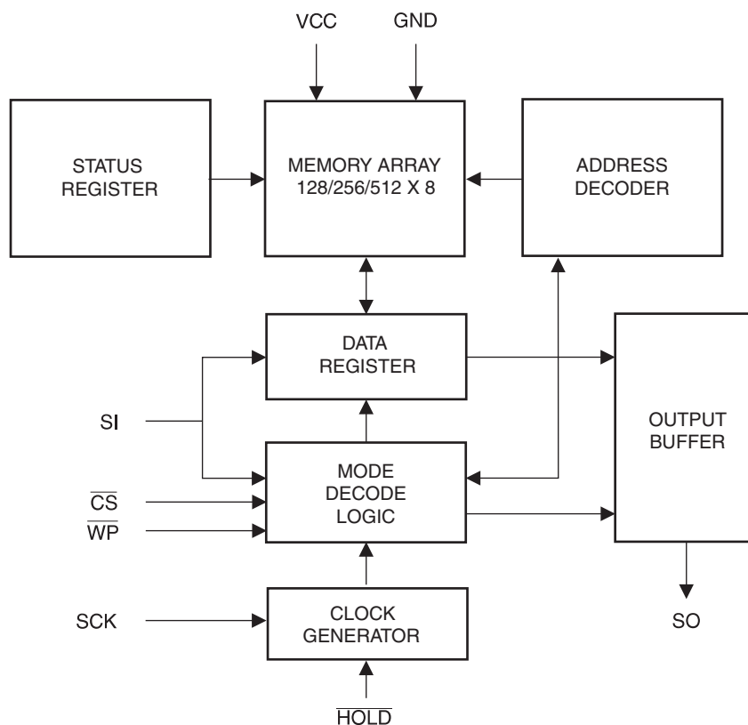
Figure 1. Block Diagram
