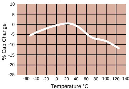
X7R Dielectric Typical Temperature Coefficient
