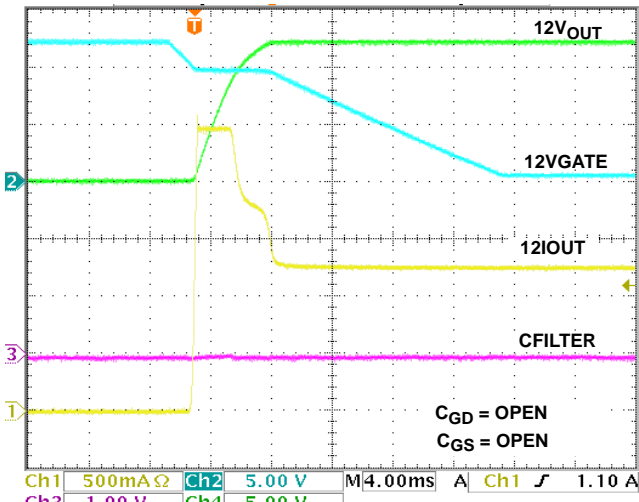
FIGURE 10. ISL6114 12VMAIN START-UP R LOAD = 10Ω, C LOAD = 470μF
