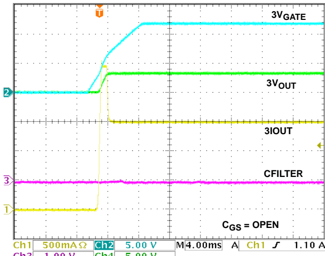
FIGURE 11. ISL6114 3VMAIN START-UP R LOAD = 2Ω, C LOAD = 470μF
