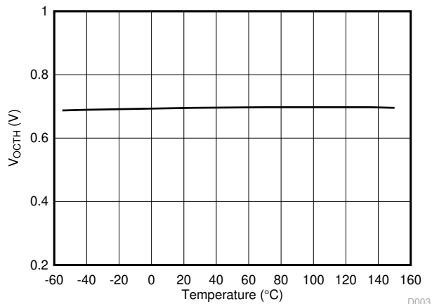
Figure 5-25. V_{OCOFF} OC Detection Threshold vs Temperature
