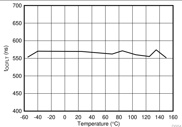
Figure 5-26. t_{OCOFF} OC to FLT Low Delay Time vs Temperature
