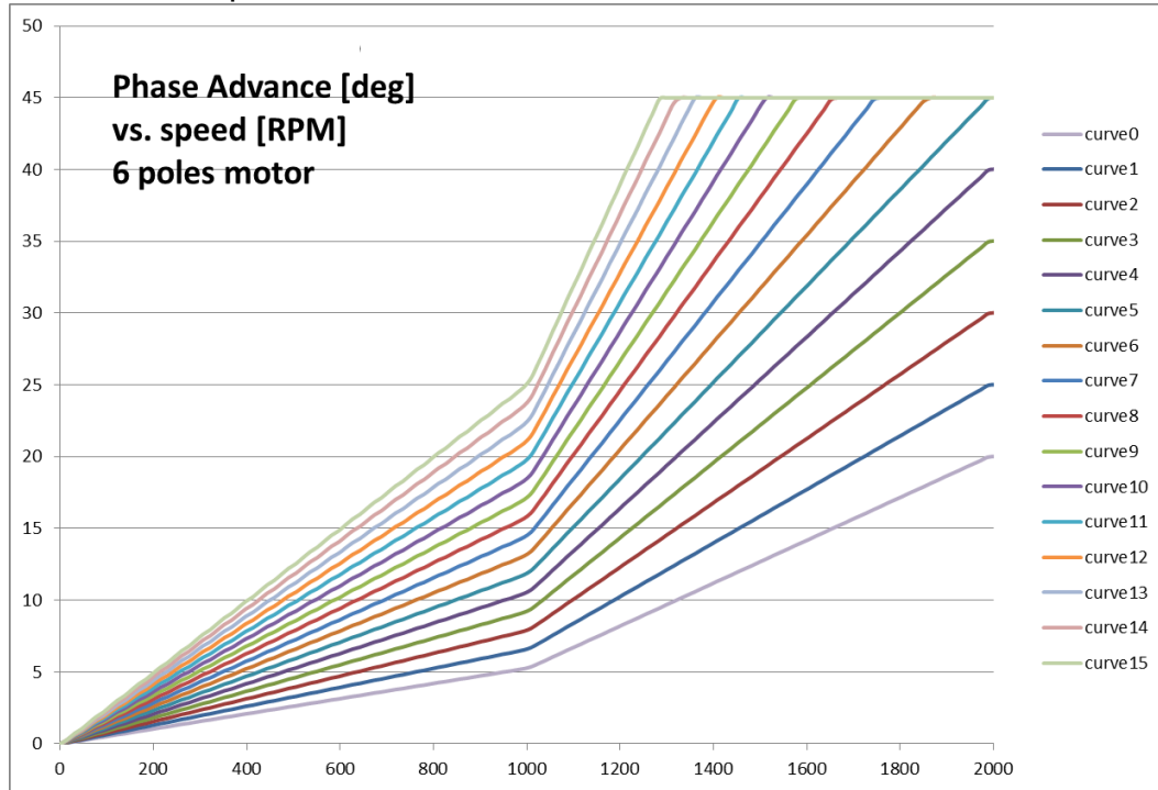
Load curves for 6 poles motor
