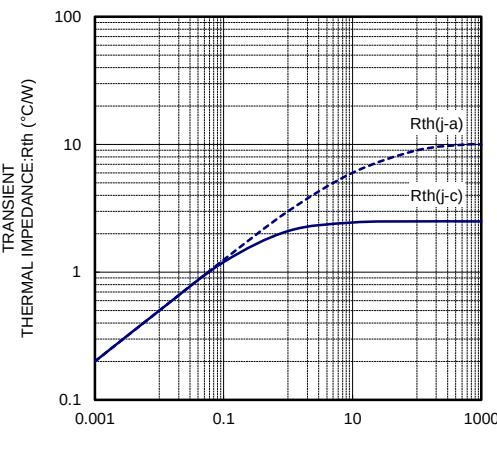
R_th-t CHARACTERISTICS
