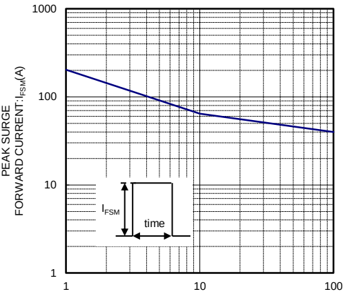
I_FSM-t CHARACTERISTICS
