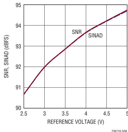
SNR, SINAD vs Reference Voltage, f_{IN} = 2\text{kHz}
