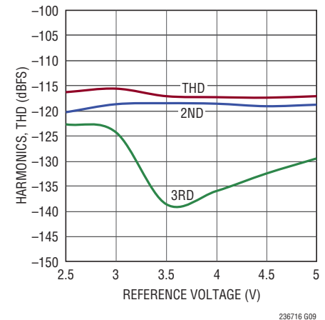
THD, Harmonics vs Reference Voltage, f_{IN} = 2\text{kHz}
