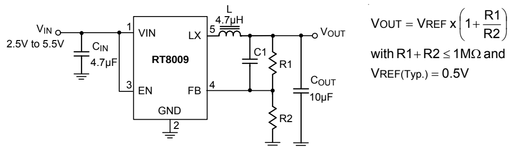
Figure 2. Adjustable Voltage Regulator
