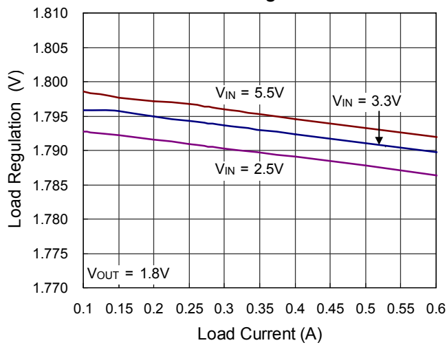
Load Regulation
