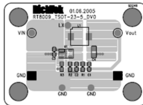
Figure 7. Top Layer
