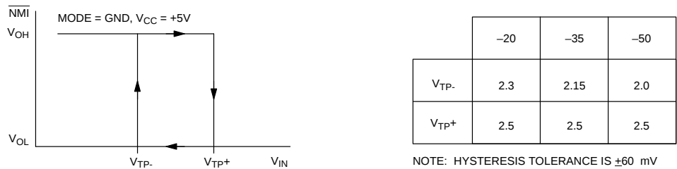
INPUT PIN HYSTERESIS Figure 3
