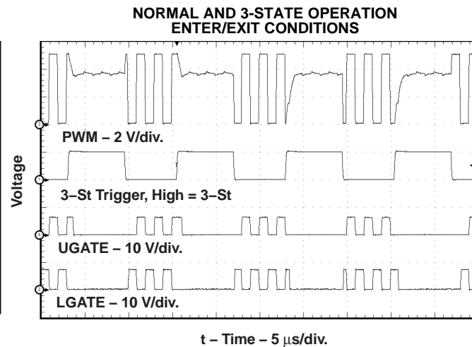
Figure 18. The 3-state upper threshold reverts to the 2-V level after the TPS28226 had been in 3-state for about 2.5 μs.
