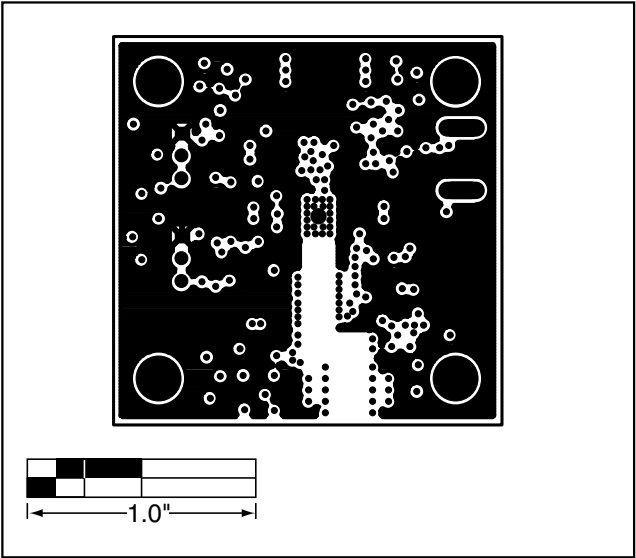
Figure 12. MAX2266 EV Kit PC Board Layout—Power Plane
