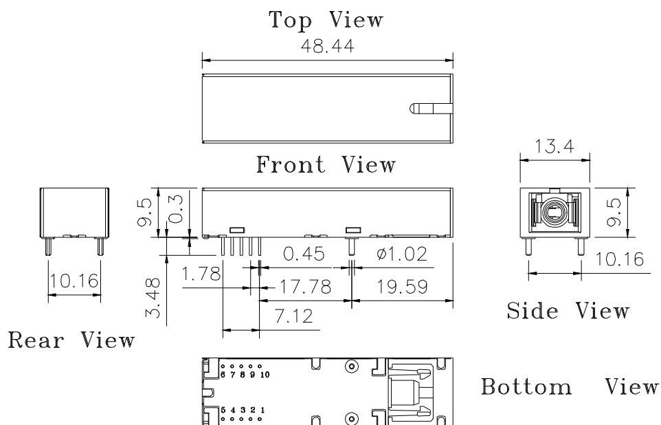
BTRS-5780-1510G
