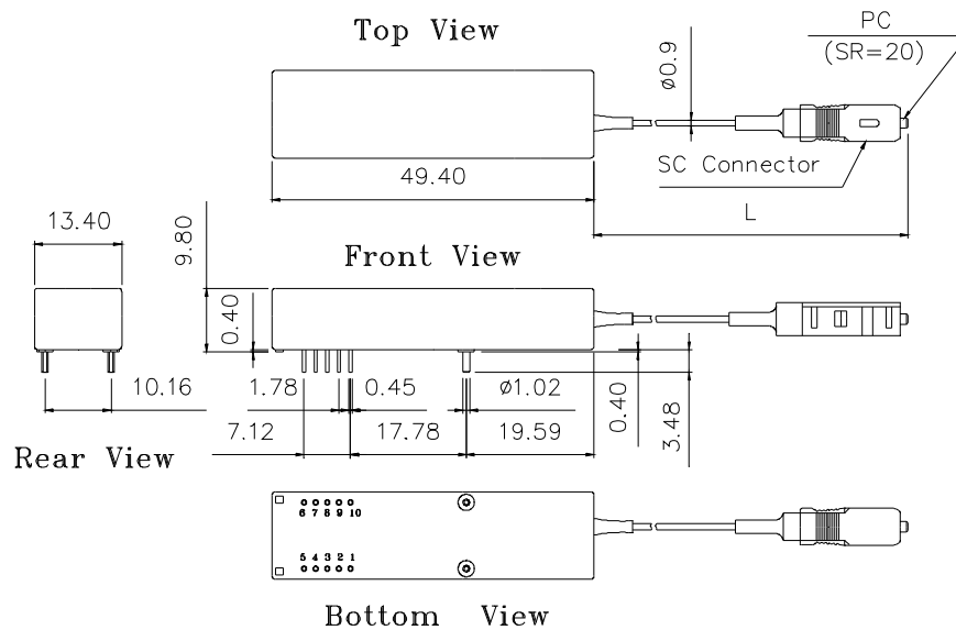
BTRS-5780-1510-SP50G
