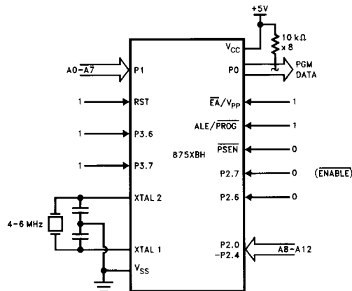
Figure 10. Verifying the EPROM
