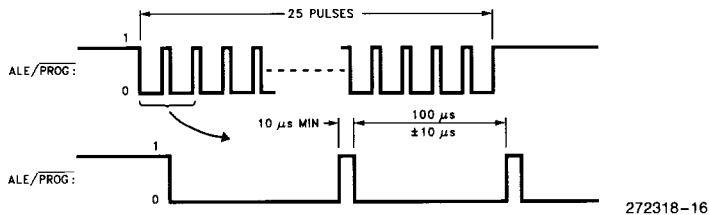
Figure 9. PROG Waveforms
