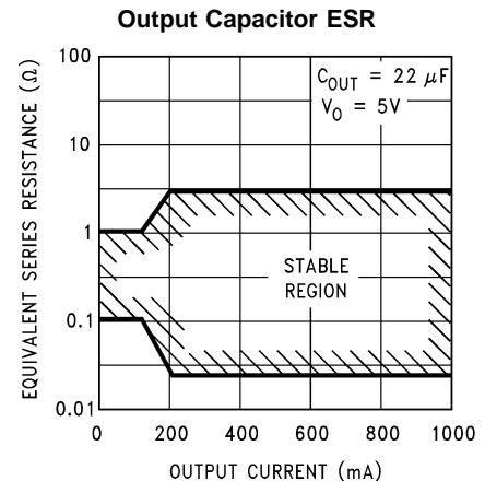
FIGURE 1. ESR Limits
