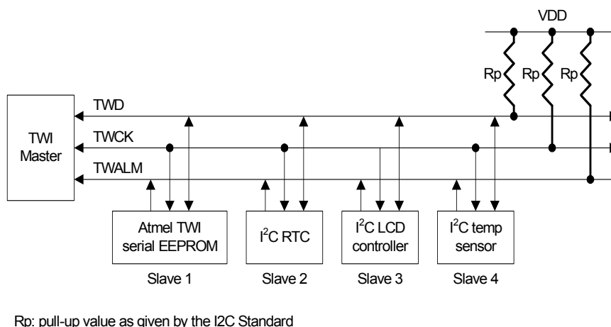
Figure 23-2. Application Block Diagram
