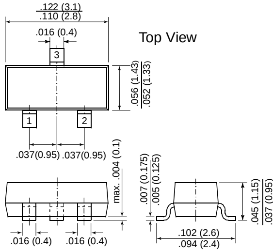
TO-236AB (SOT-23)
