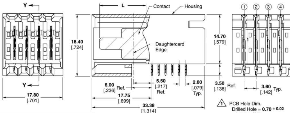
Section Y-Y
