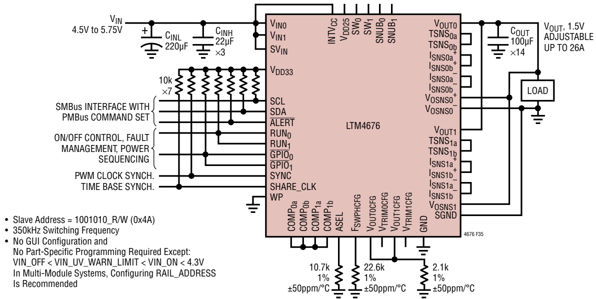
Figure 35. 26A, 1.5V Output DC/DC \mu Module Regulator with I 2 C/SMBus/PMBus Serial Interface
