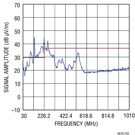
Figure 32. Radiated Emissions Scan of LTM4676 Producing 1V OUT at 26A, from 12V IN . DC1811 Hardware with Outputs Paralleled. No Snubbers Applied. f_{SW} = 350 kHz. Measured in a 10m Chamber. Peak Detect Method
