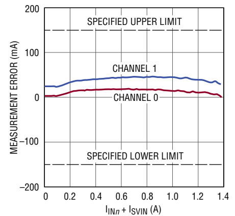
MFR_READ_IIN n (Input Current Readback) Error vs ( I_{\text{VIN}n} + I_{\text{SVIN}} ), FCM, I_{\text{OUT}n} Swept from 0\text{A} to 13\text{A} , One Channel at a Time, \text{RUN}_{1-n} = 0\text{V}
