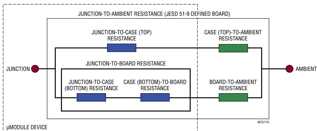
Figure 10. Graphical Representation of JEESD51-12 Thermal Coefficients
