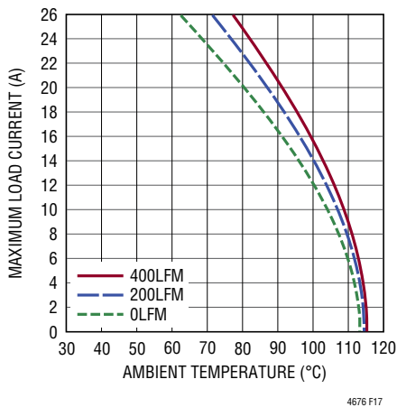
Figure 17. 5V to 1V Derating Curve, BGA Heat Sink
