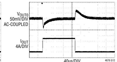
FIGURE 44 CIRCUIT AT 24\text{V}_{\text{IN}} , \text{C}_{\text{OUT}0} = 5 \times 100\mu\text{F} AND \text{VOUT}_0 COMMANDED TO 3.300\text{V} . 0\text{A} TO 10\text{A} LOAD STEP AT 10\text{A}/\mu\text{s}
