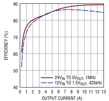
Single Phase Single Output Burst Mode Efficiency, \text{V}_{\text{IN}} = \text{SV}_{\text{IN}} = \text{V}_{\text{INn}} , \text{INTV}_{\text{CC}} Open, \text{MFR\_PWR\_MODE}_n[1:0] = 01_b
