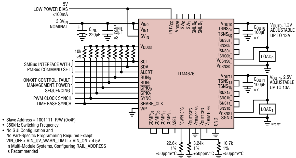
Figure 37. 13A, 1.2V and 2.5V Outputs Generated from 3.3V Power Input and Providing I 2 C/SMBus/PMBus Serial Interface
