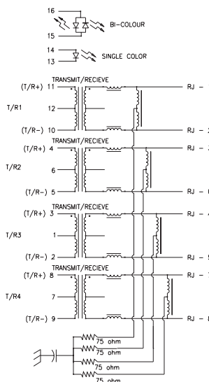
SCHEMATIC (RJMG-B3XX-71-01), CAP. 1000pF, 2KV
