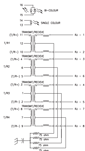
SCHEMATIC (RJMG-B3XX-81-01), CAP. 1000pF, 2KV
