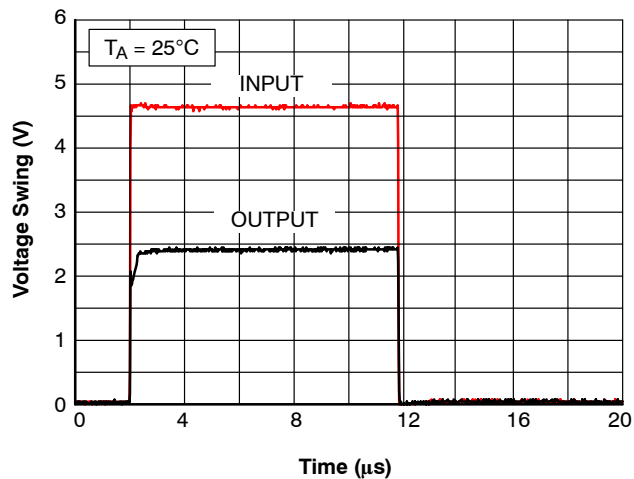
Figure 16. Pulse Response
