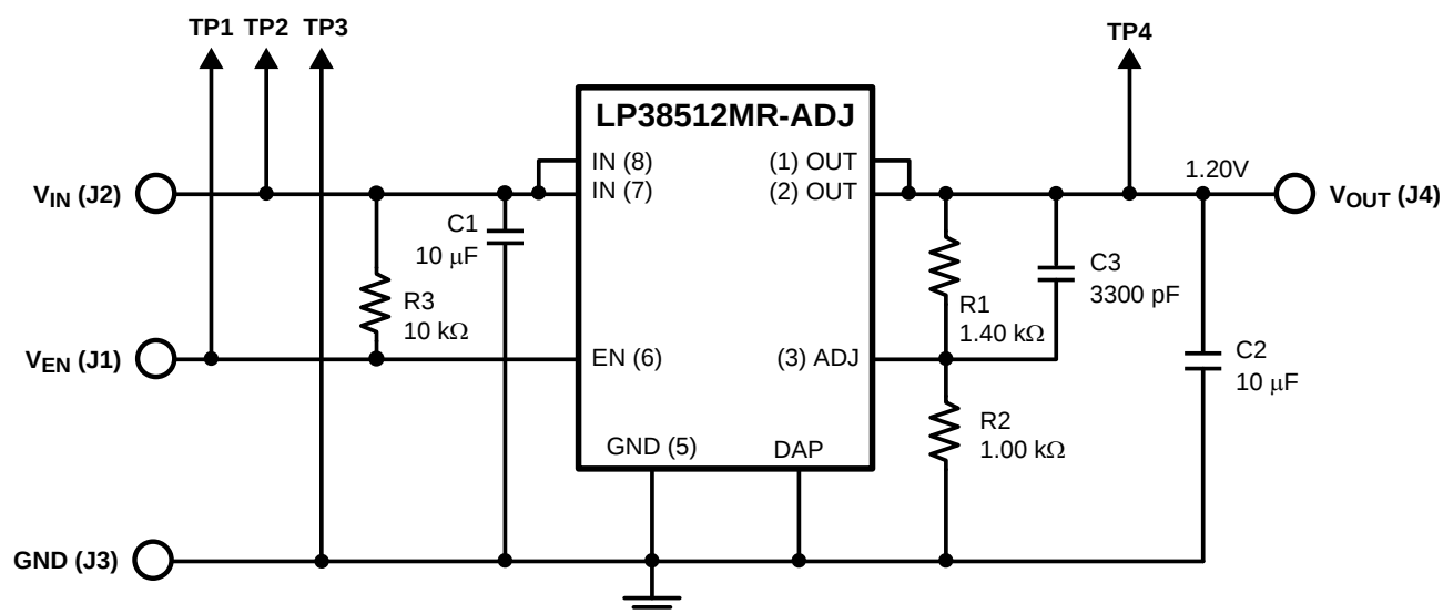
Figure 7. Evaluation Board Schematic.
