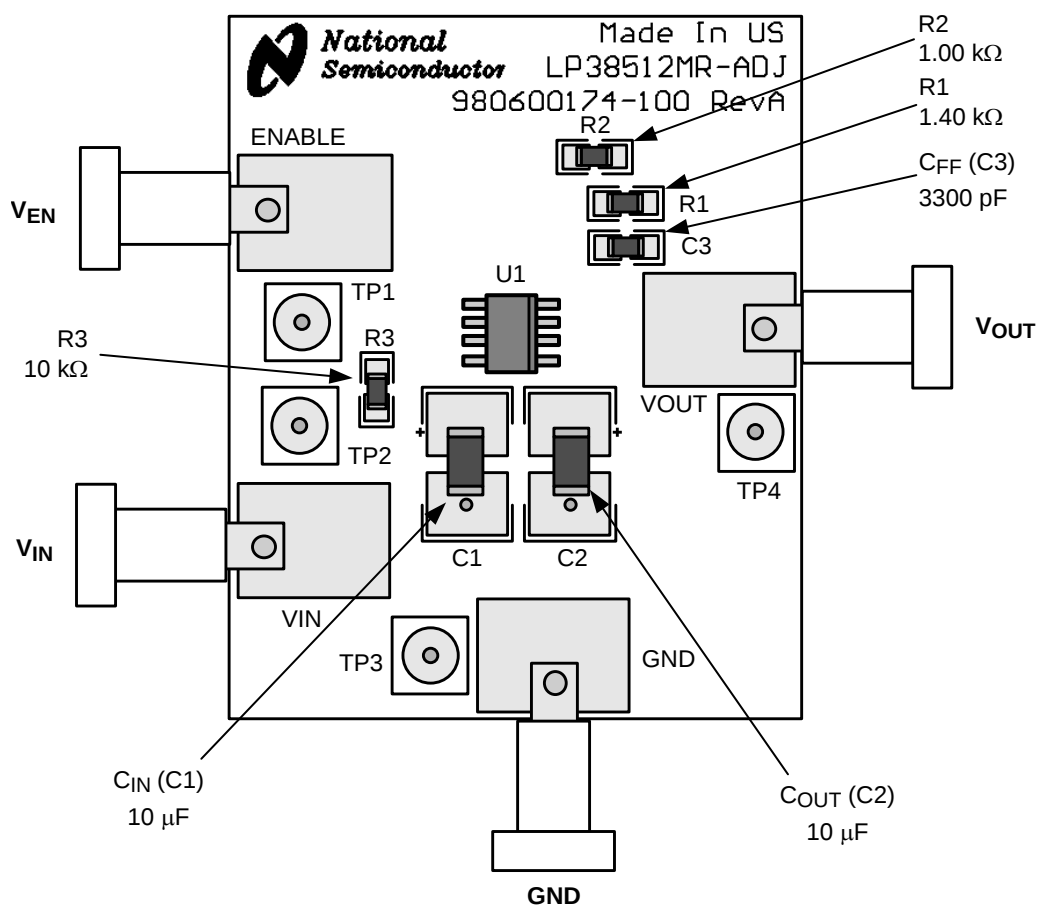
Figure 8. Evaluation Board Component and Pin Layout
