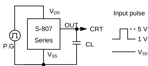
(b) CMOS output products
