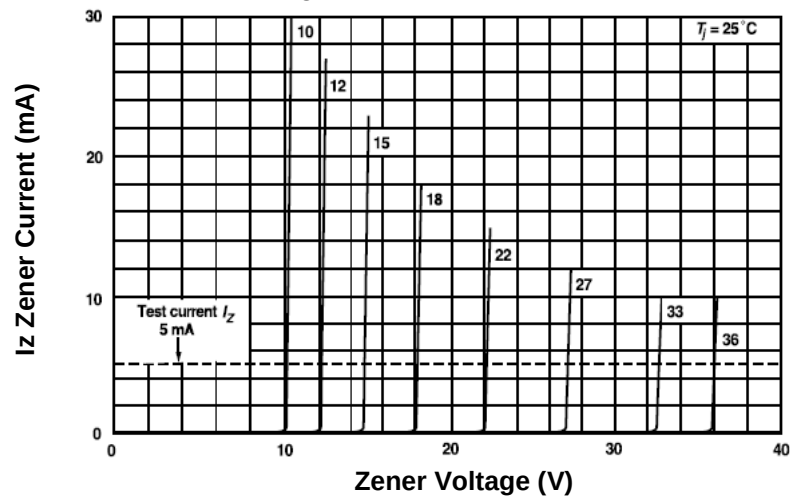
Fig.3 Breakdown Characteristics
