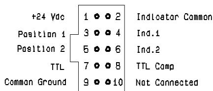
Switch connector
