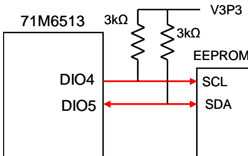
Figure 35: EEPROM Connection
