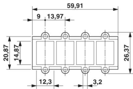
RJ45 panel mounting frame, IP20
