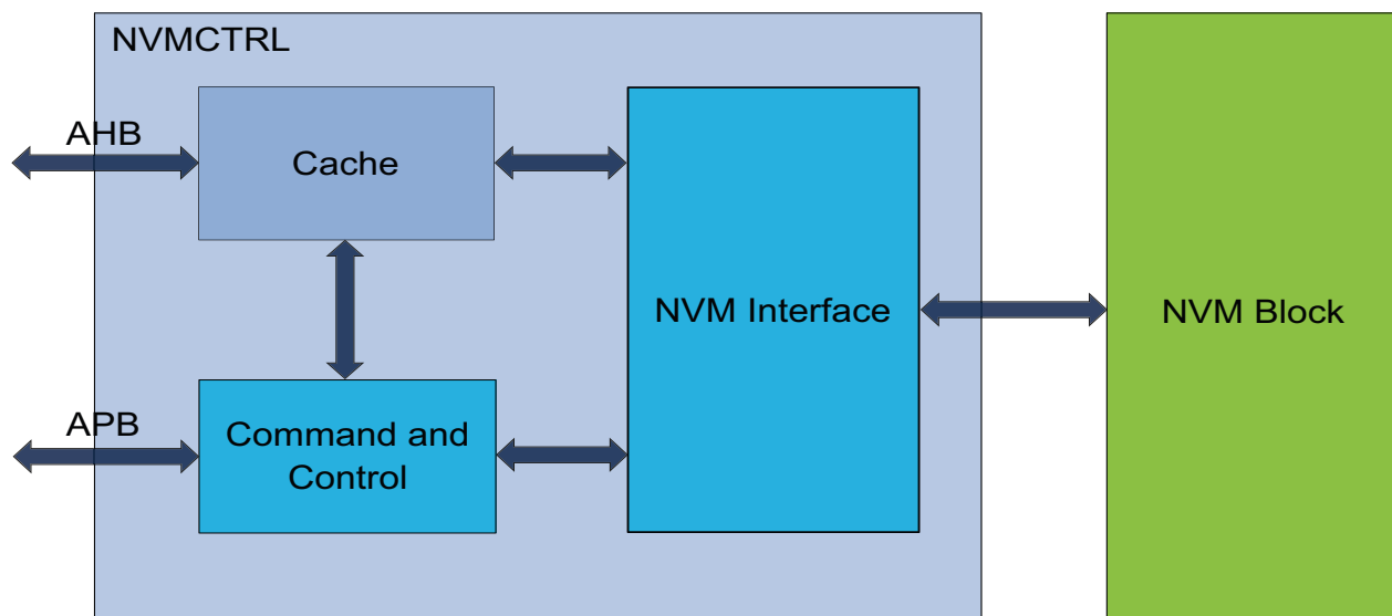
Figure 21-1. Block Diagram
