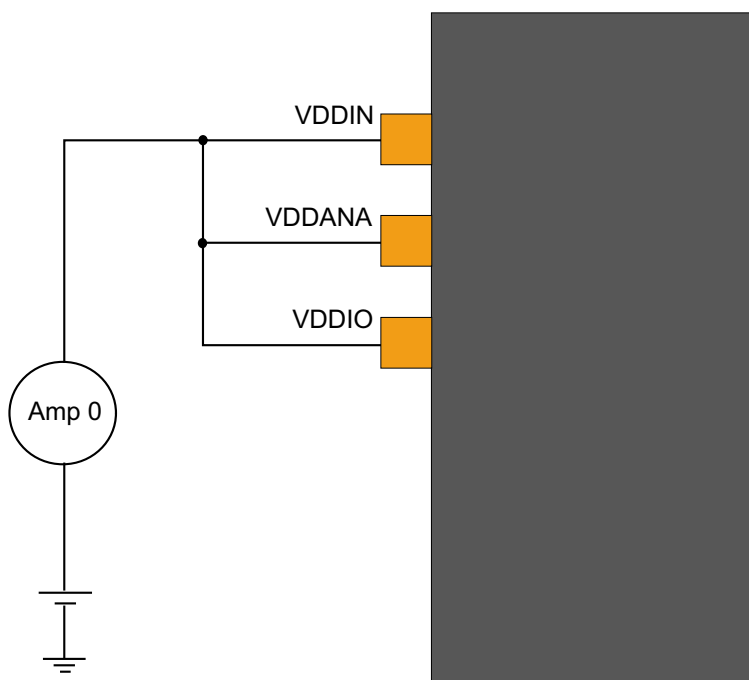
Figure 40-1. Measurement Schematic
