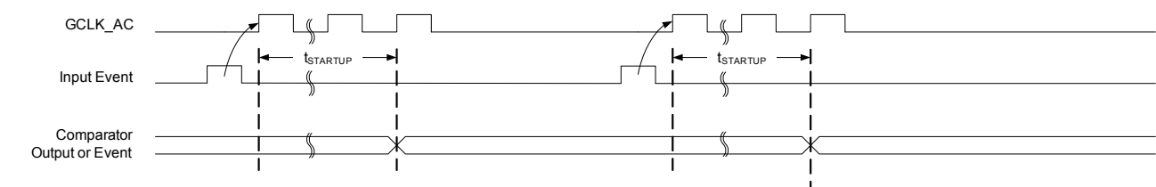
Figure 32-10. Single-Shot SleepWalking
