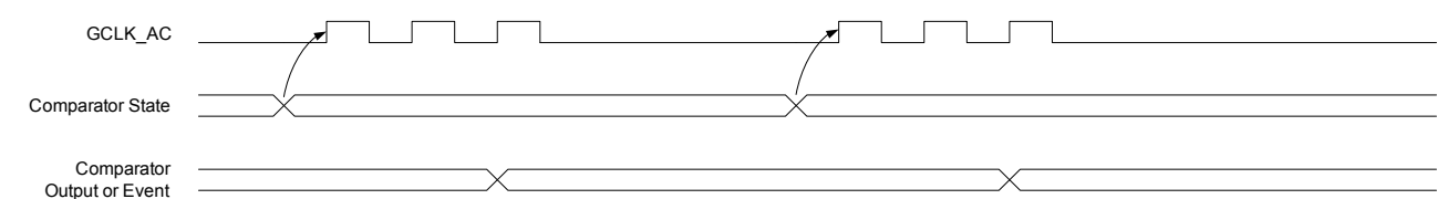
Figure 32-9. Continuous Mode SleepWalking
