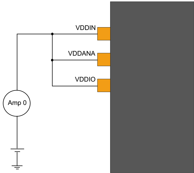
Figure 35-1. Measurement Schematic
