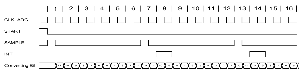
Figure 31-5. ADC Timing for Free Running in Differential Mode without Gain
