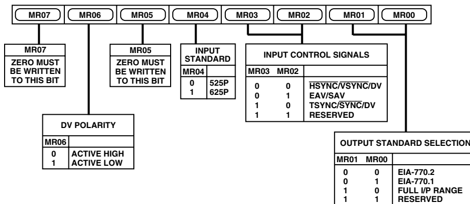
Figure 16. Mode Register 0
