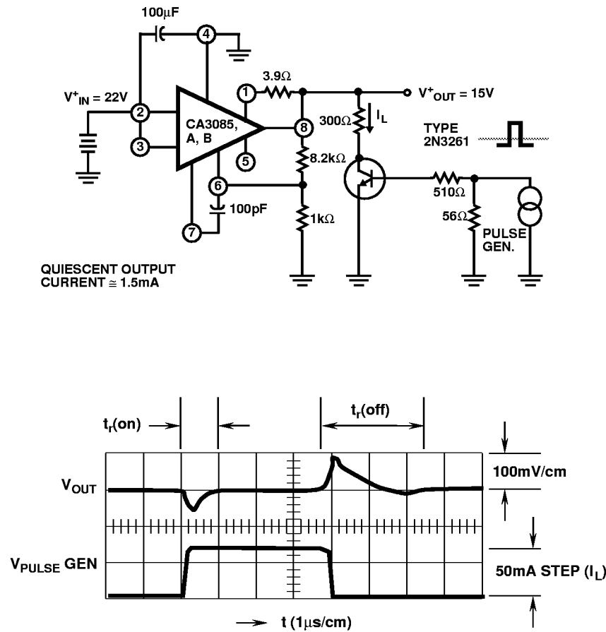
FIGURE 16. TURN-ON AND TURN-OFF RECOVERY TIME TEST CIRCUIT WITH ASSOCIATED WAVEFORMS
