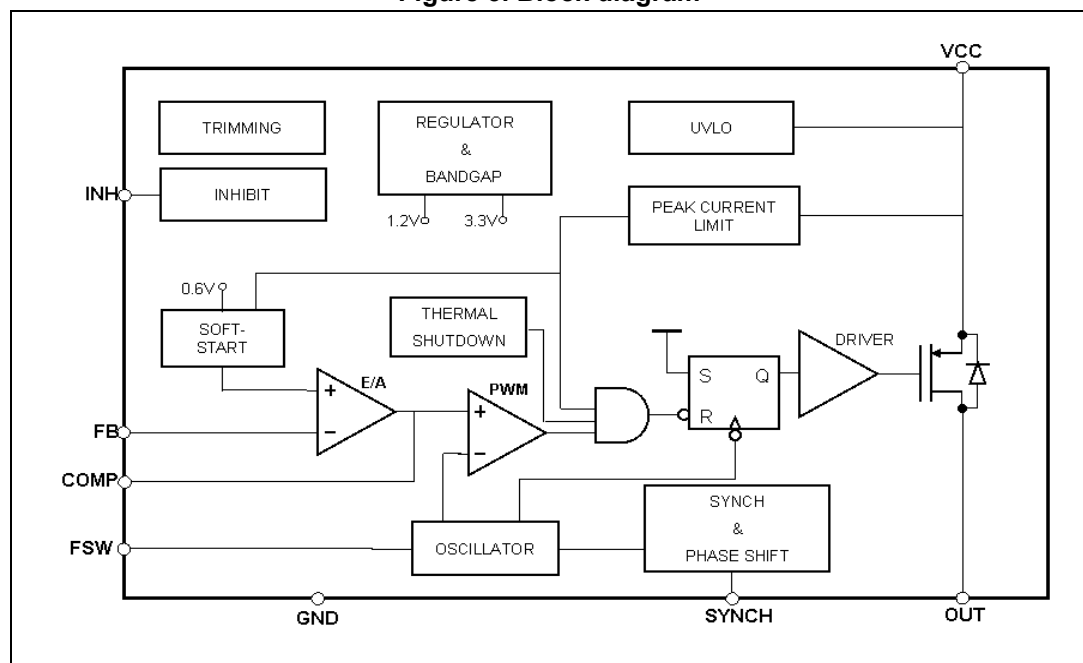
Figure 3. Block diagram
