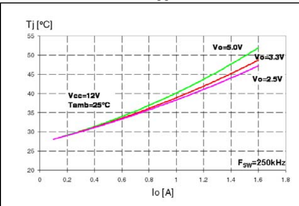
Figure 23. Junction temperature vs. output current - V_{CC} = 12\text{ V}
