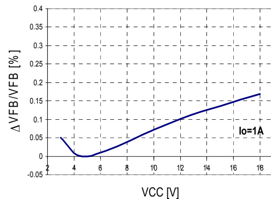
Figure 29. Line regulation
