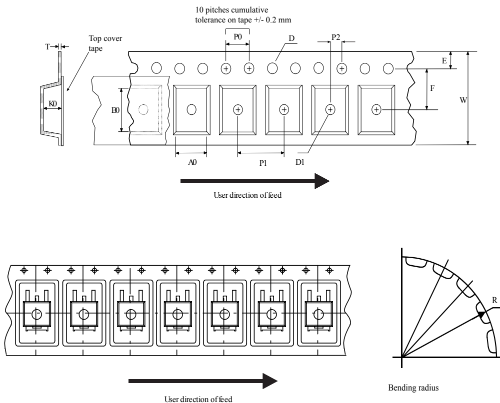
Figure 28. Tape outline
