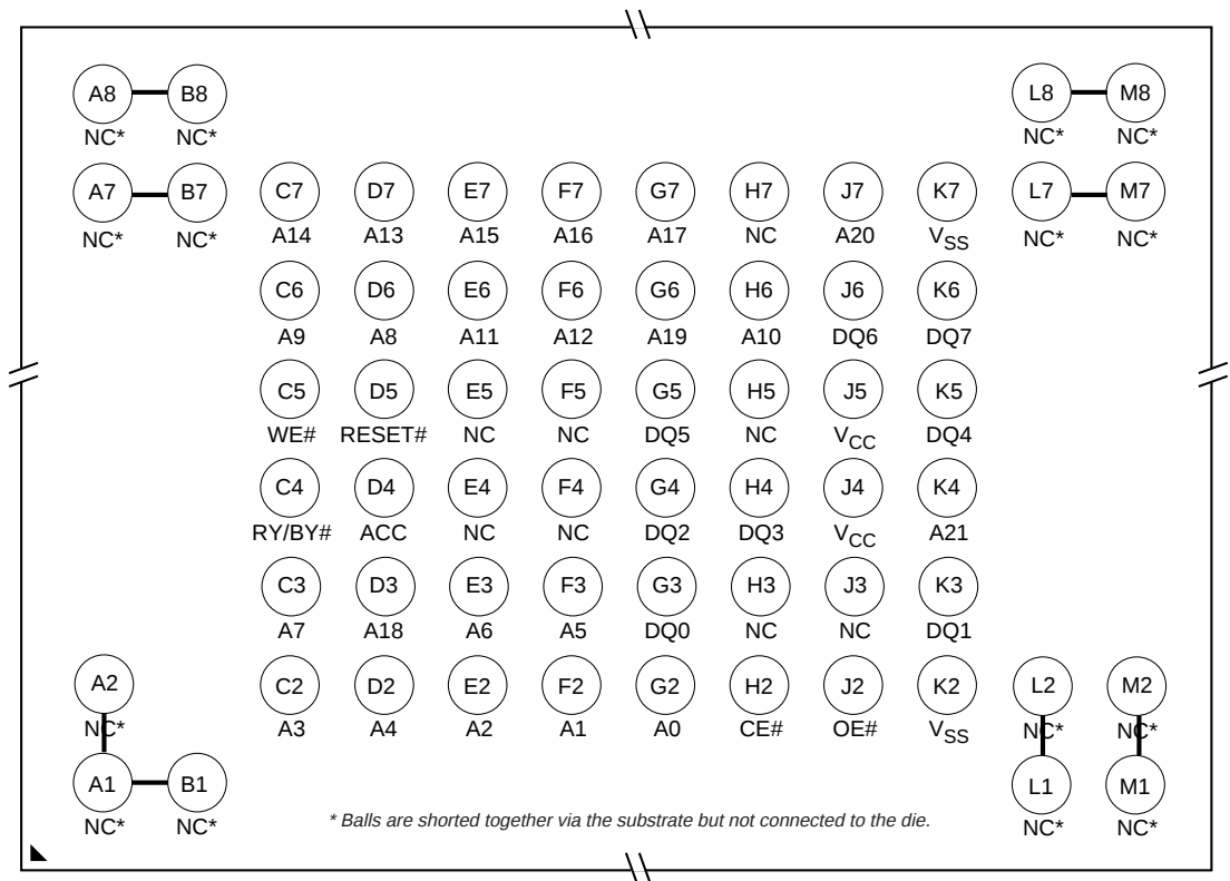
63-Ball FBGA (Top View, Balls Down)
