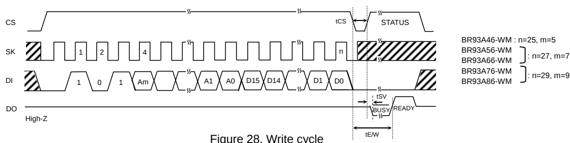
Figure 28. Write cycle
