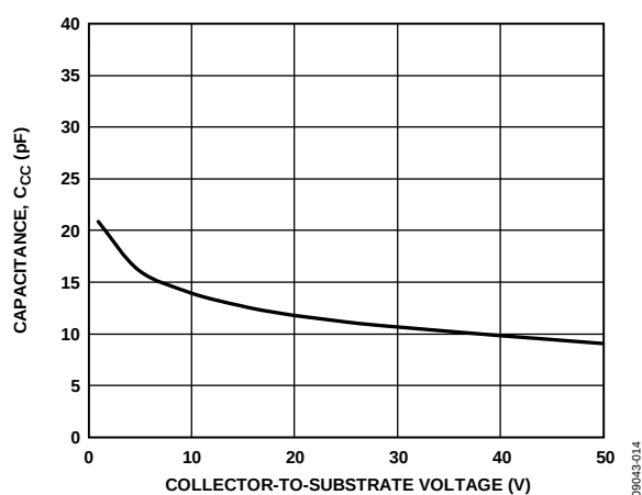
Figure 14. Collector-to-Collector Capacitance vs. Collector-to-Substrate Voltage
