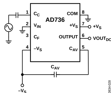
Figure 23. Low-Z AC-Coupled Input Connection
