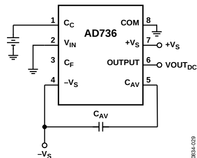
Figure 24. Low-Z DC-Coupled Input Connection
