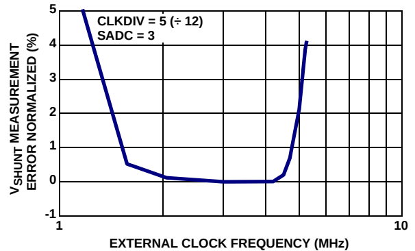
FIGURE 37. EXTERNAL CLOCK BANDWIDTH vs MEASUREMENT ACCURACY
