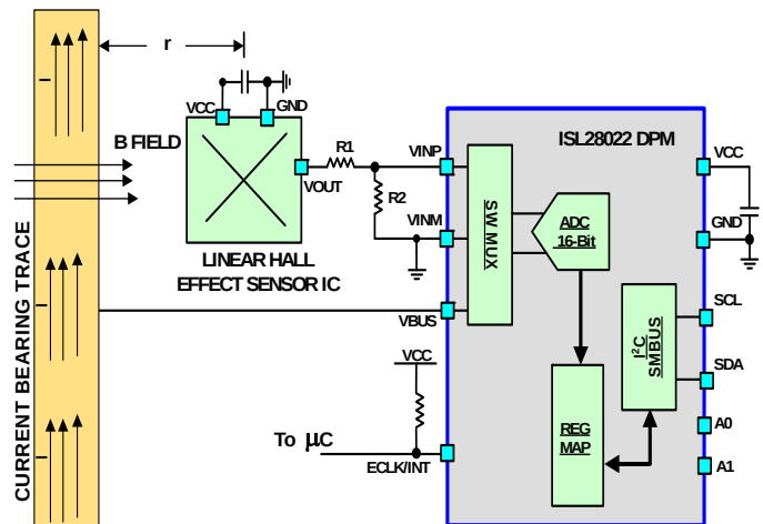
FIGURE 55. A SIMPLIFIED CIRCUIT DIAGRAM OF REMOTELY MEASURING CURRENT THROUGH A TRACE
