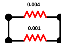
FIGURE 38. A SIMPLIFIED SCHEMATIC ILLUSTRATING THE USE OF TWO SHUNT RESISTORS TO CREATE A DESIRED SHUNT VALUE
