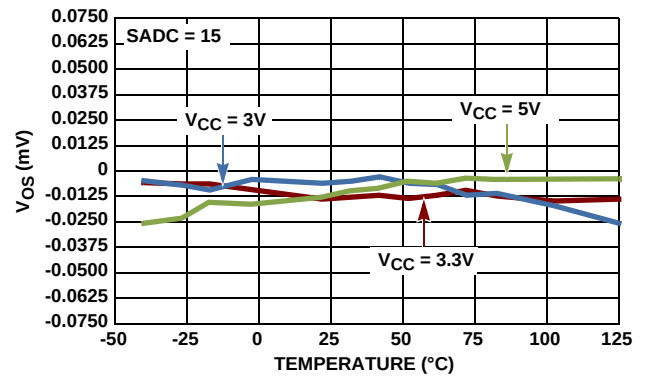
FIGURE 3. V_{SHUNT} V_{OS} vs TEMPERATURE
