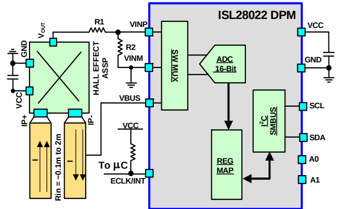
FIGURE 57. A SIMPLIFIED CIRCUIT DIAGRAM OF A HALL EFFECT SENSOR THAT INTEGRATES THE CURRENT CONDUCTION PATH
