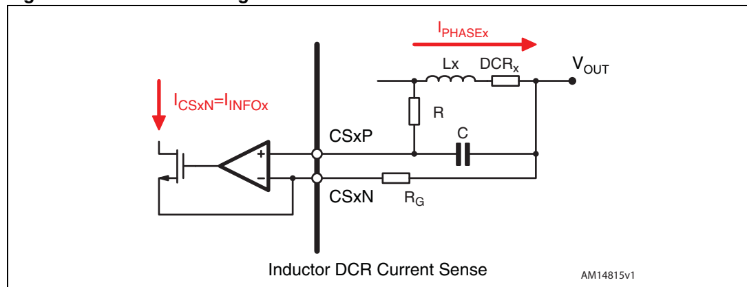
Figure 7. Current reading
