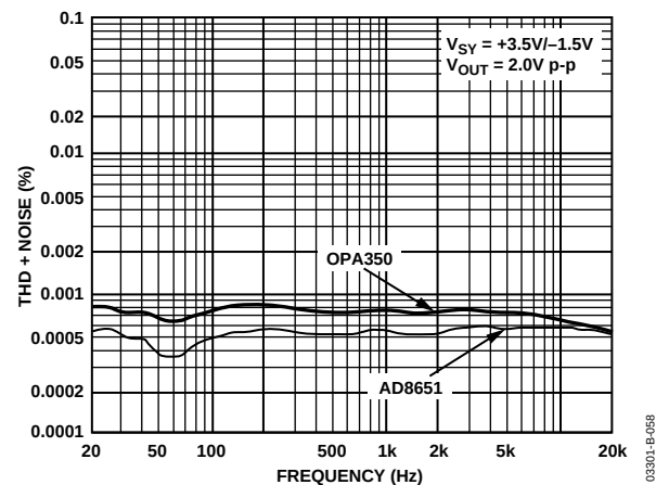
Figure 57. Total Harmonic Distortion
