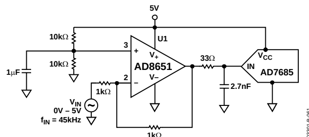
Figure 60. AD8651 Driving a 16-Bit ADC
