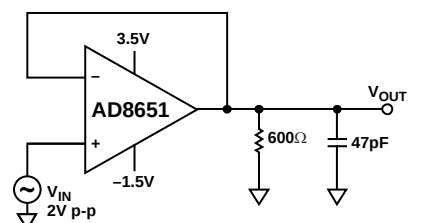
Figure 58. THD + N Test Circuit
