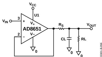
Figure 55. Driving Large Capacitive Loads
