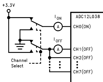
Figure 19. Leakage Current
