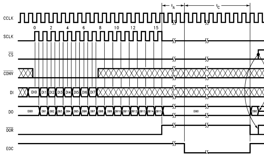
Figure 31. ADC12L038 Conversion with \overline{\text{CS}} Continuously Low and 16-Bit Digital Output Format
