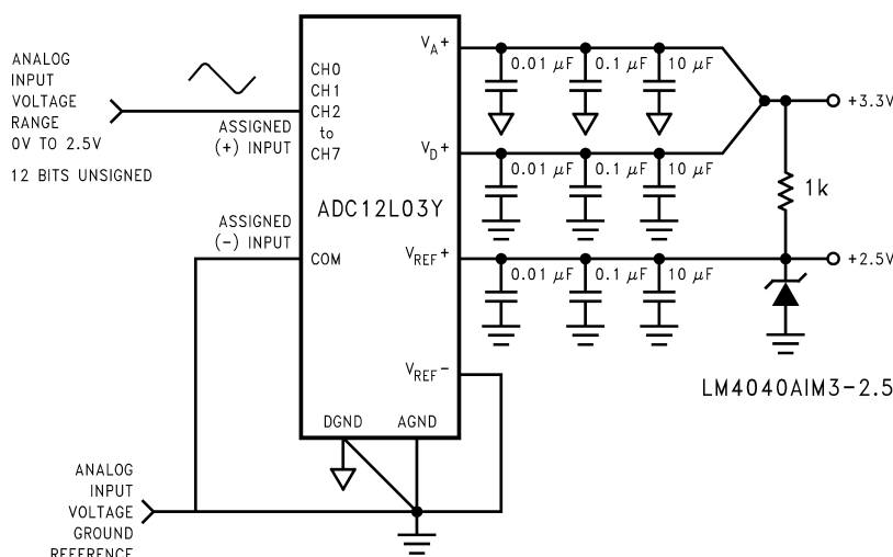
Figure 42. Single-Ended Biasing
