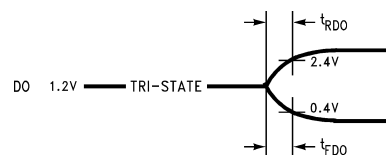
Figure 21. DO "TRI-STATE" Falling and Rising Edge
