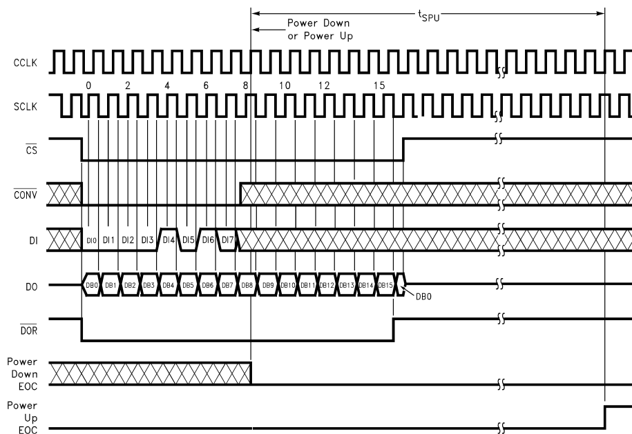
Figure 32. ADC12L038 Software Power Up/Down Using \overline{\text{CS}} with 16-Bit Digital Output Format
