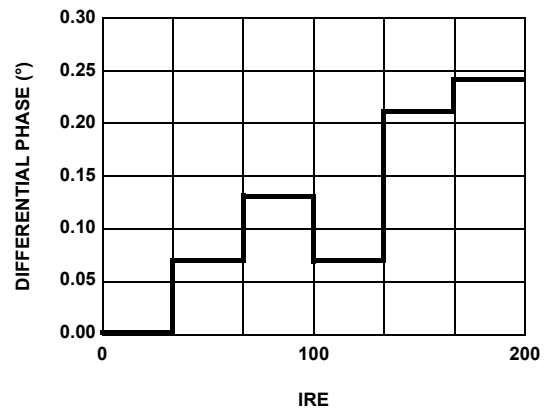
FIGURE 12. DIFFERENTIAL PHASE
