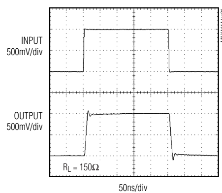
MAX4414/MAX4416/MAX4418 LARGE-SIGNAL PULSE RESPONSE
