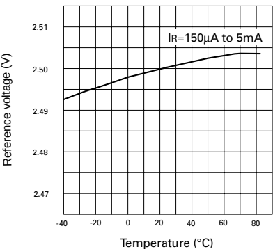
Temperature Drift
