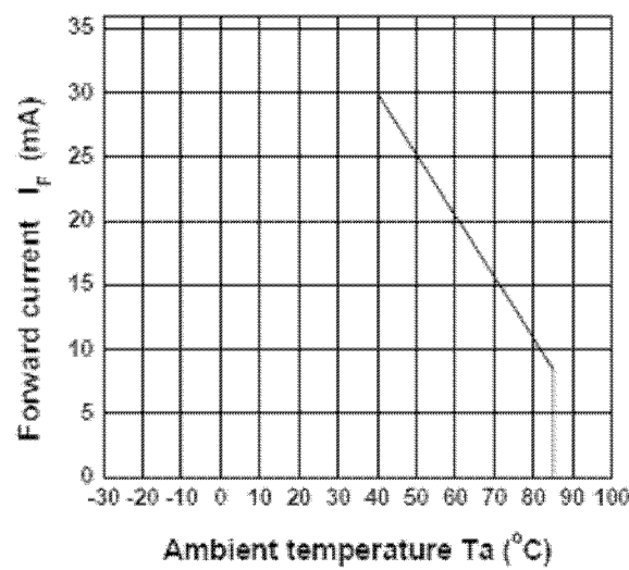
Diode IF-Ta CHARACTERISTICS DIAGRAM
