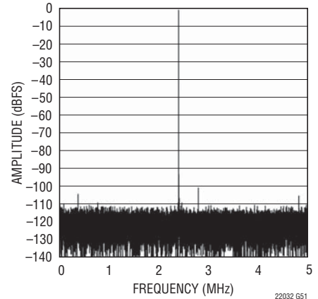
LTC2202: 32K Point FFT, f_{IN} = 12.4\text{MHz} , -1\text{dBFS} , PGA = 0
