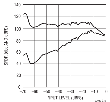
LTC2203: SFDR vs Input Level, f_{IN} = 70.1\text{MHz} , \text{PGA} = 0 , Dither "Off"
