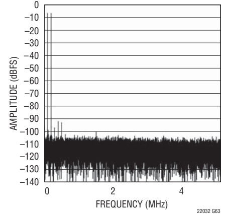
LTC2202: 32K Point 2-Tone FFT, f_{IN} = 60.2\text{MHz} and 70.1\text{MHz} , -7\text{dBFS} , \text{PGA} = 0
