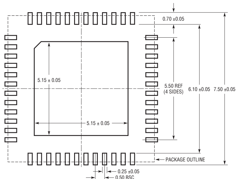
UK Package 48-Lead Plastic QFN (7mm × 7mm) (Reference LTC DWG # 05-08-1704)
