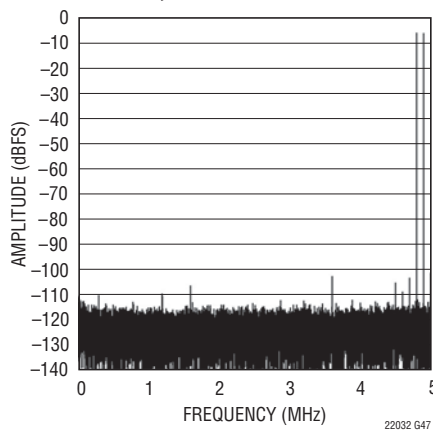
LTC2202: 32K Point 2-Tone FFT, f_{IN} = 5.1\text{MHz} and 15.2\text{MHz} , -7\text{dBFS} , PGA = 0
