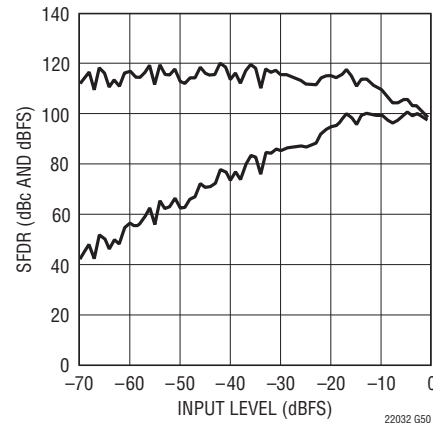
LTC2202: SFDR vs Input Level, f_{IN} = 5\text{MHz} , PGA = 0, Dither "On"
