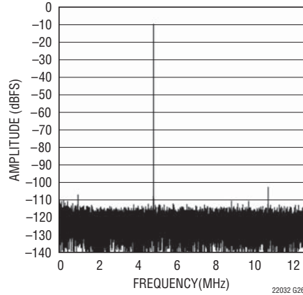
LTC2203: 32K Point FFT, f_{IN} = 70.1\text{MHz} , -10\text{dBFS} , \text{PGA} = 1
