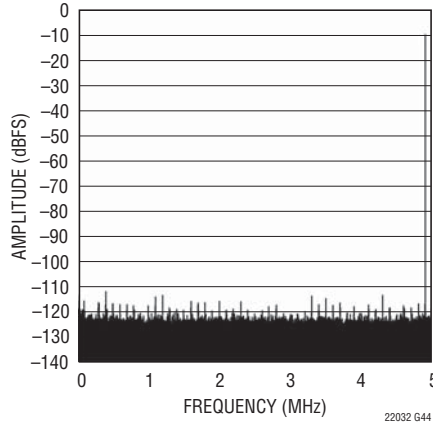
LTC2202: 128K Point FFT, f_{IN} = 5.1\text{MHz} , -10\text{dBFS} , PGA = 0
