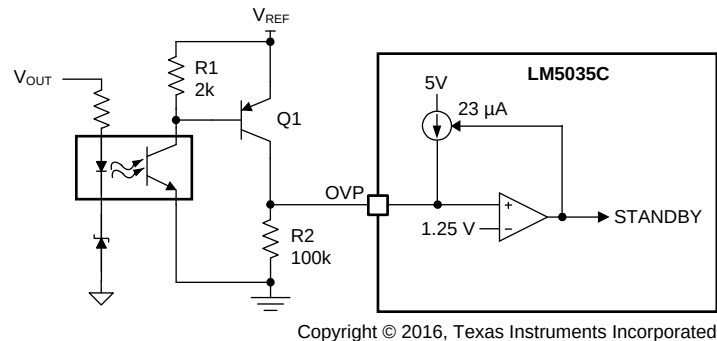
Figure 24. Latched Load Overvoltage Protection
