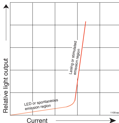
Figure 15. Relative light output versus input current of a laser diode.
