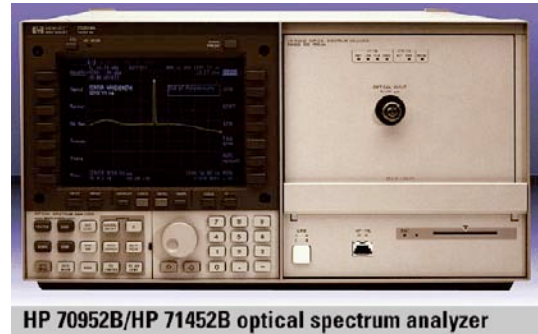
Photo 13. An optical spectrum analyzer is used to characterize the light outputs from LEDs and lasers.
